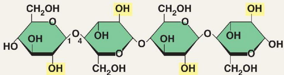
Cellulose: 1-4 linkage of \beta glucose monomers
